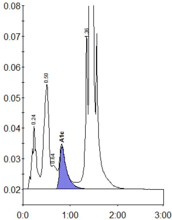
Peak table - ID: 10644031
